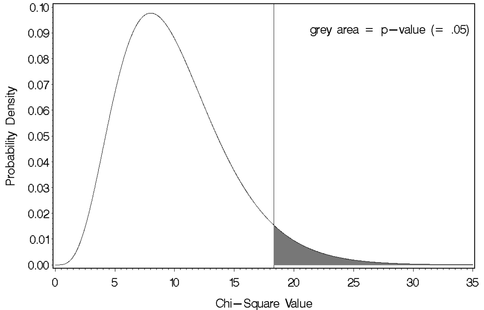
Chi-Square Distribution, df = 10
